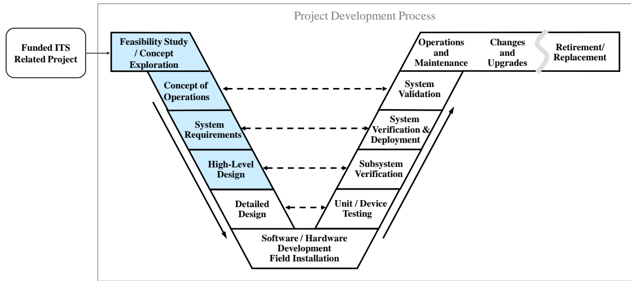
Figure 2: Use of Virginia NR ITS Architecture in the Project Development Process
