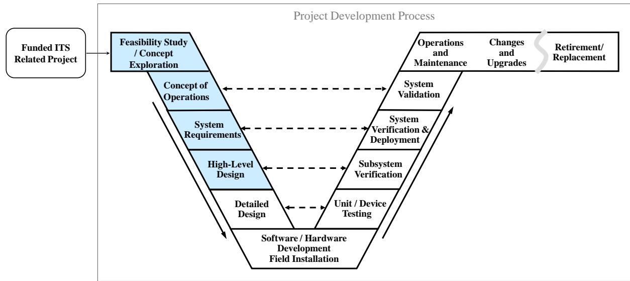
Figure 2: Use of Virginia SWR ITS Architecture in the Project Development Process
