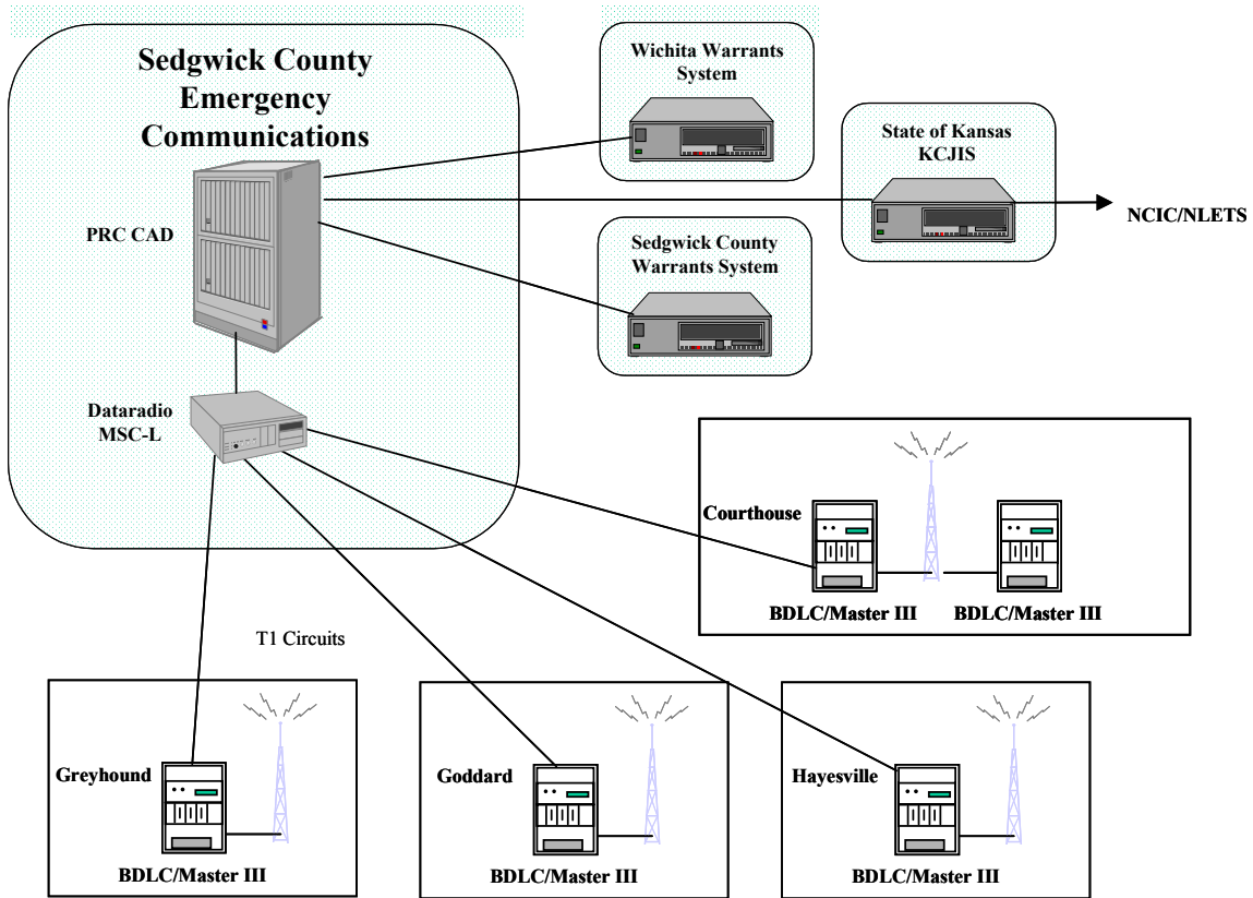
Figure 89. Mobile Data System
