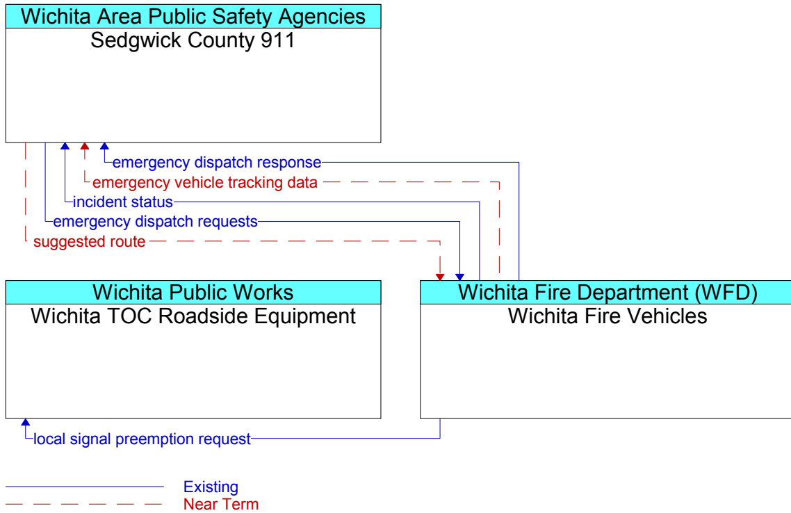
Figure 72. Wichita Fire Vehicles Communications Diagram
