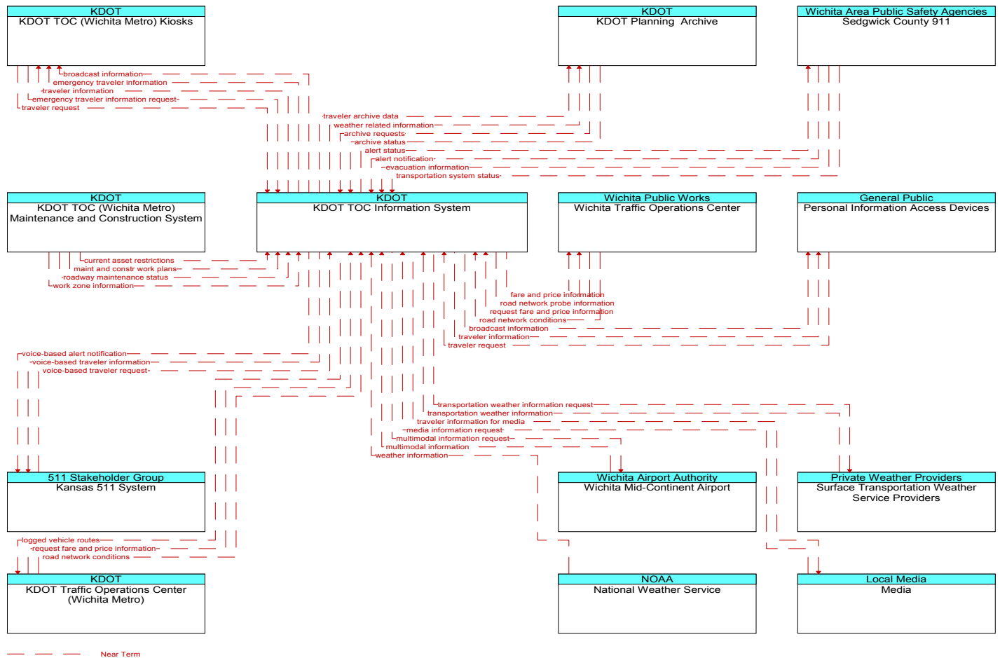
Figure 24. KDOT TOC Information System Communications Diagram
