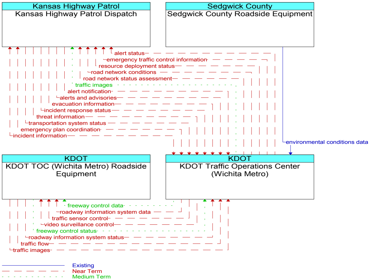
Figure 31. KDOT Traffic Operations Center (Wichita Metro) Communications Diagram (Part 2)
