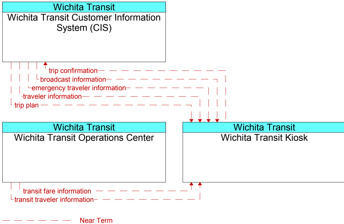
Figure 82. Wichita Transit Kiosk Communications Diagram
