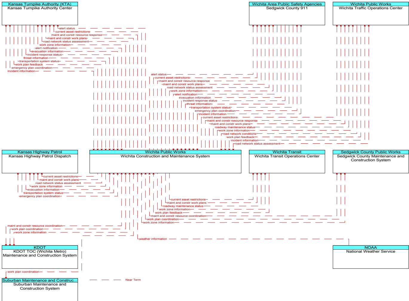
Figure 69. Wichita Construction and Maintenance System Communications Diagram (Part 1)
