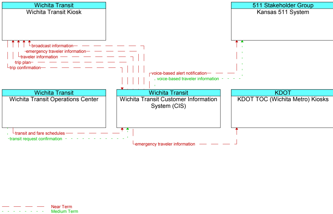
Figure 81. Wichita Transit Customer Information System (CIS) Communications Diagram
