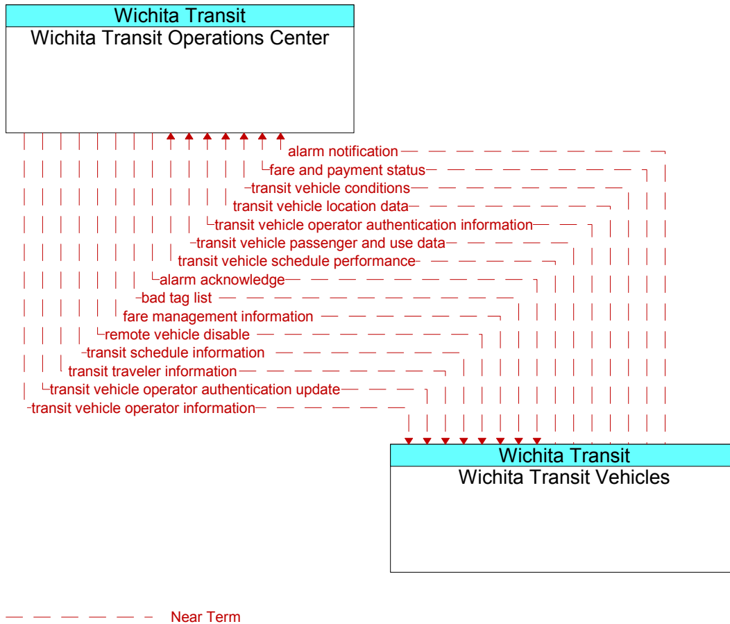
Figure 86. Wichita Transit Operations Center Communications Diagram (Part 4)
