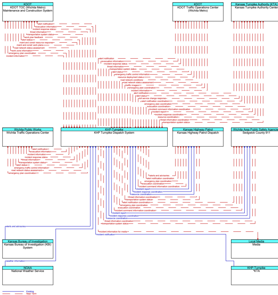
Figure 33. KHP Turnpike Dispatch System Communications Diagram (Part 1)
