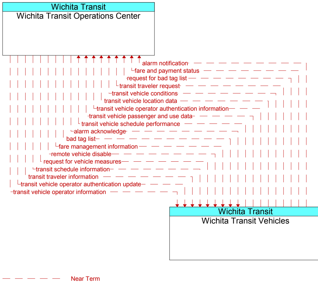
Figure 87. Wichita Transit Vehicles Communications Diagram
