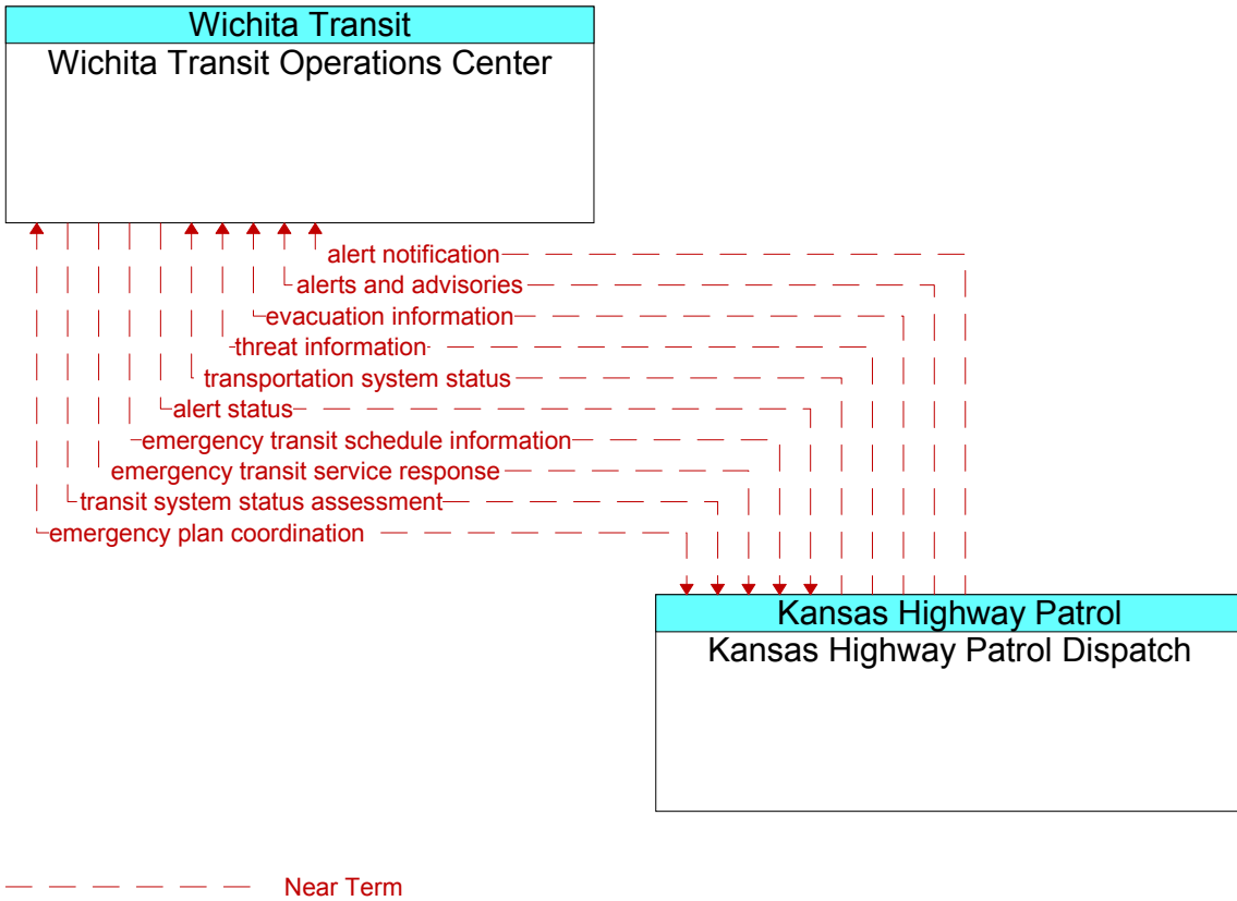
Figure 84. Wichita Transit Operations Center Communications Diagram (Part 2)
