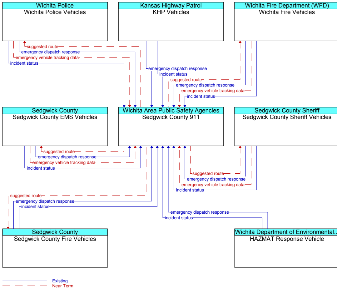
Figure 50. Sedgwick County 911 Diagram (Part 3)
