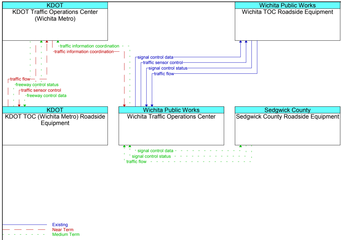
Figure 3. Regional Traffic Control Architecture Flow Diagram
